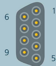
Micro-D Connector Pin Assignment (Front View)
